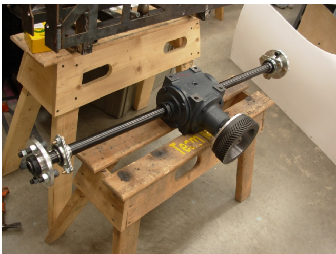
Rear Axle
